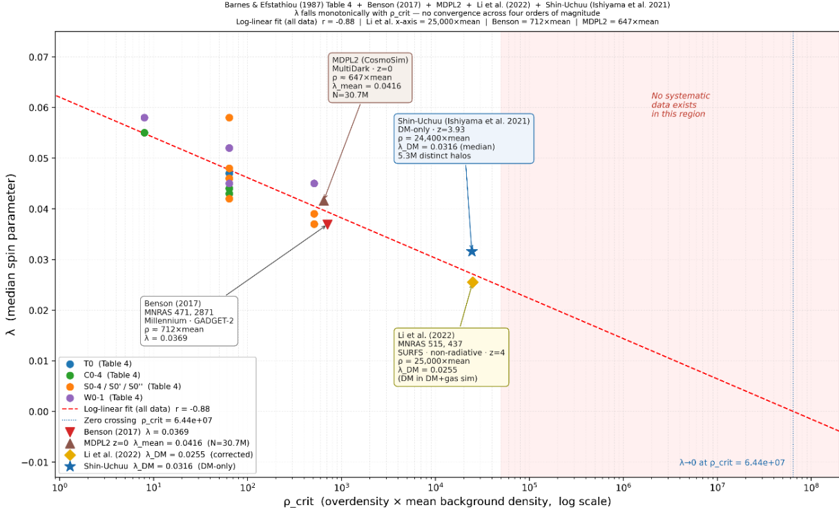
Figure 4. Halo spin parameter \lambda vs overdensity threshold \rho_{crit} . Barnes & Efstathiou (1987). Benson (2017), Li et al. (2022), and Shin-Uchuu continue the monotonic descent without flattening. Li et al. x-axis = 25,000 \times \text{mean} at z = 0 , derived from \Delta_{200} mean density definition at z = 4 . Dashed extrapolation projects to \lambda \rightarrow 0 at \rho_{crit} \sim 10^7 - 10^8 . No free parameters in the placement of the modern points. This is the empirical measurement of E[\lambda] \rightarrow 0 predicted by A.4–A.6.
